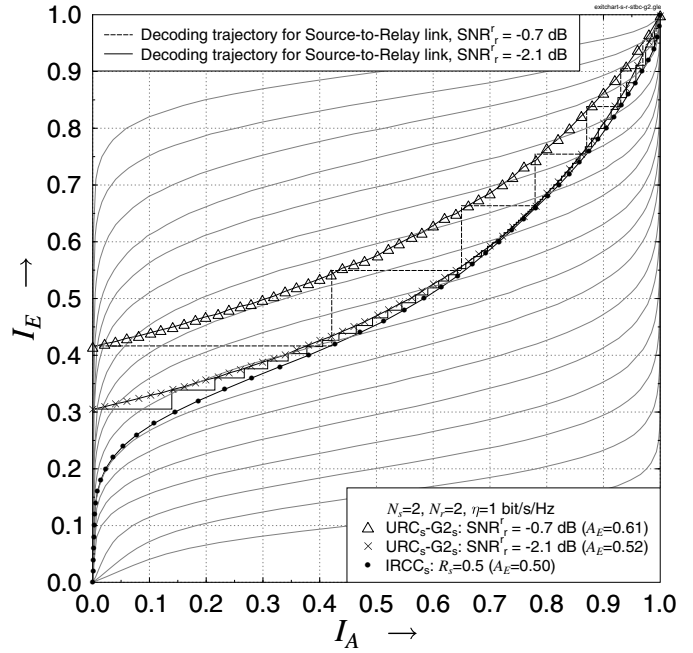
Fig. 6. The EXIT chart curves of the URC s -G 2s , the IRCC s with optimized weighting coefficients [\alpha_1, \dots, \alpha_{17}] = [0, 0, 0, 0, 0, 0, 0.327442, 0.186505, 0.113412, 0, 0.088527, 0, 0.0781214, 0.0962527, 0.0114205, 0.0346015, 0.0136955, 0.0500168] and 17 IRCC subcodes for the (2 \times 2) SR link where the \text{SNR}_r^r is the receive SNR at the relay.
