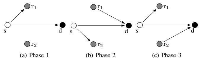
Fig. 1. System model for the successive relaying aided network, where the relays are assumed to be geographically isolated.
